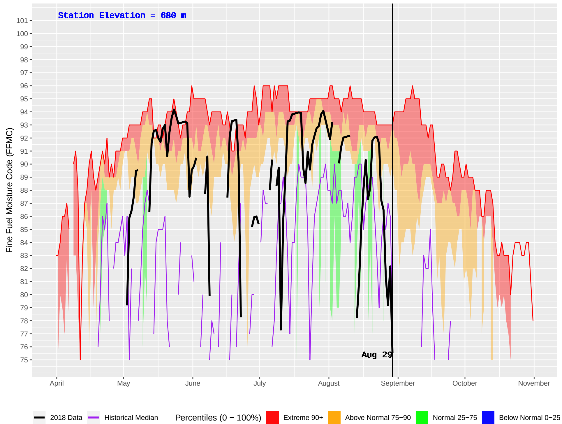
REVELSTOKE (363) : Historical (1995–2016) and Current (2018) Daily Fine Fuel Moisture Code (FFMC)
